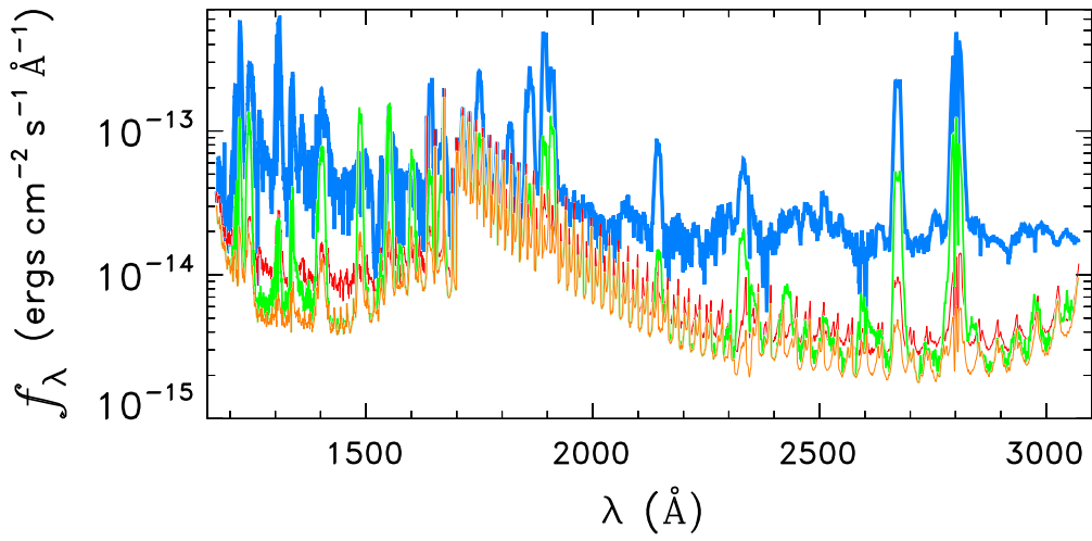
STAR0525-7014
