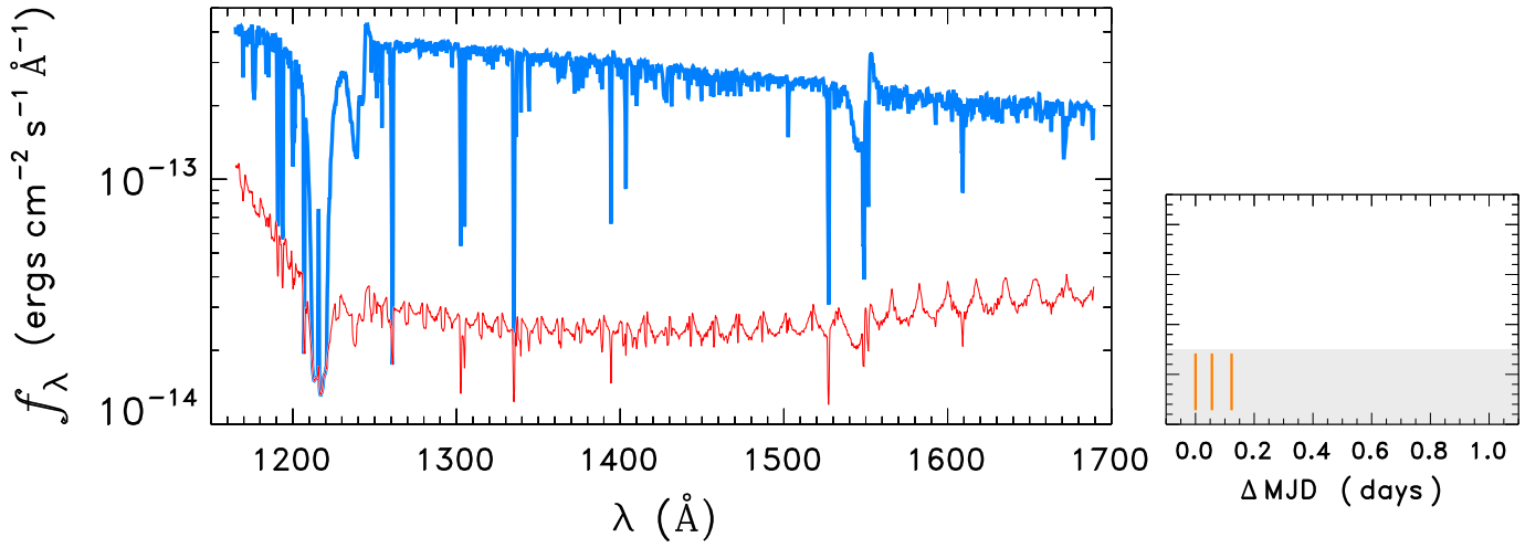
STAR0059-7205
