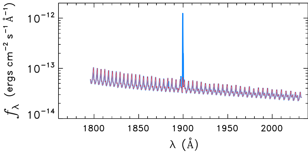
STAR0535-0523
