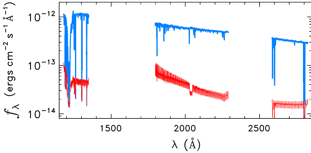
STAR0114-7320
