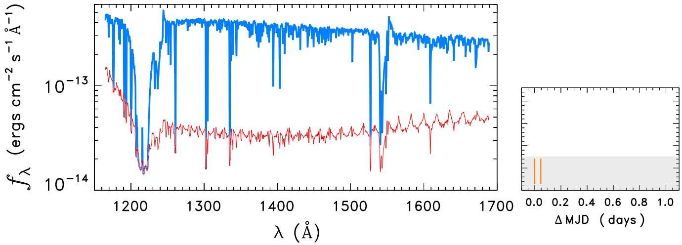
STAR0051-7244
