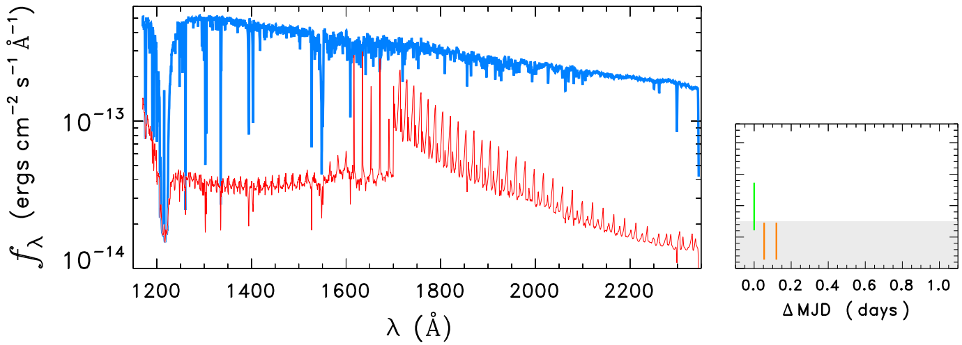
STAR0051-7248
