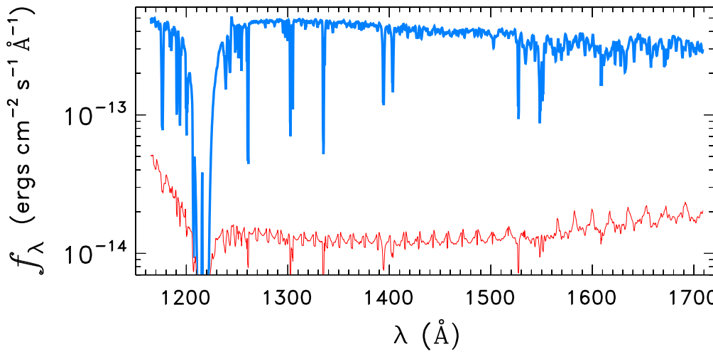
STAR0117-7326
