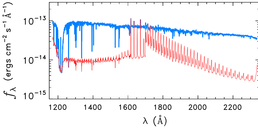
STAR0056-7227a
