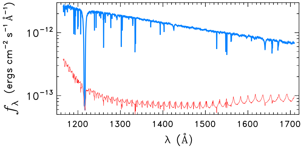
WD1957+225
