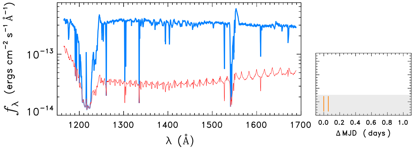
STAR0050-7247
