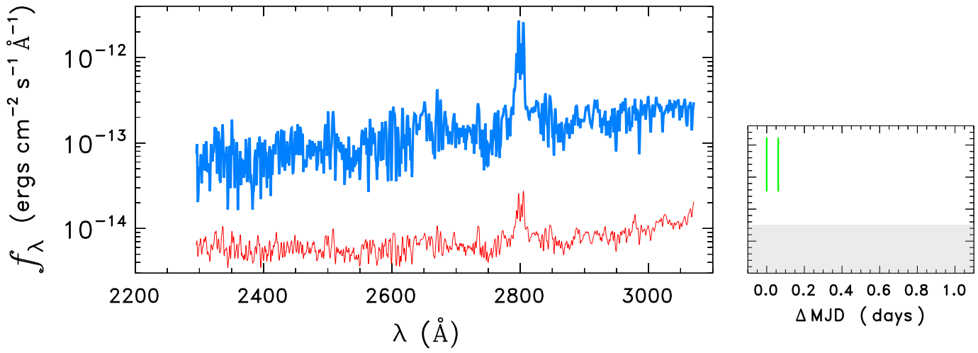
HD240764
