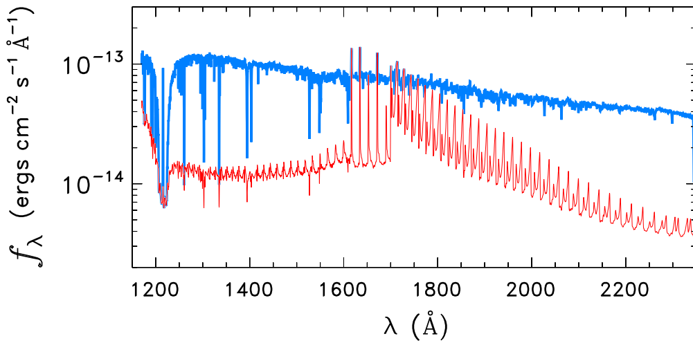
STAR0056-7227c
