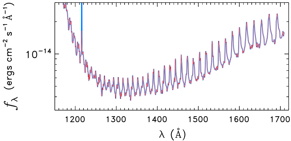
STAR0059-7210c
