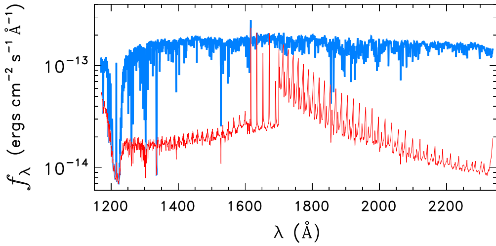
STAR0047-7307
