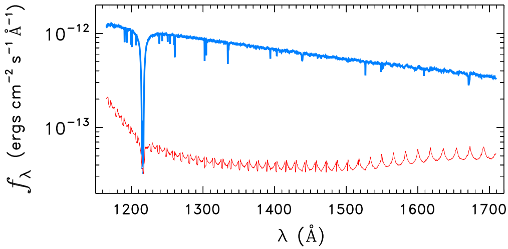
WD0939+262
