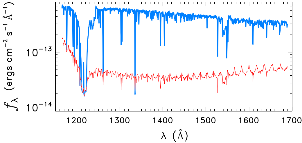
STAR0048-7325
