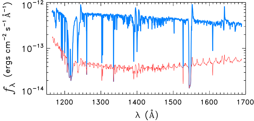
STAR0050-7242
