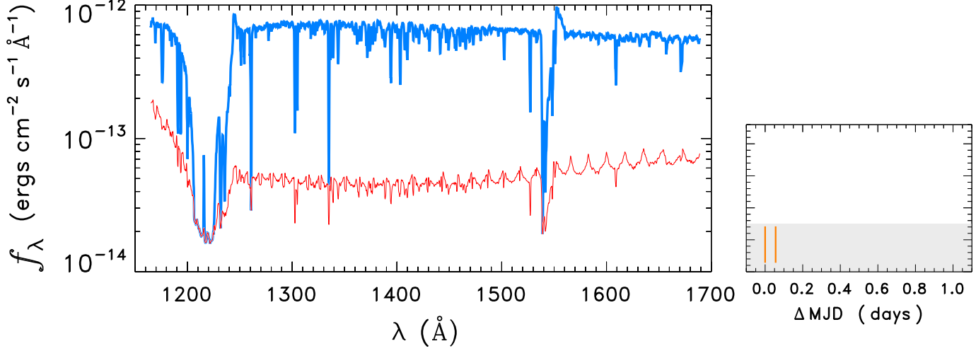
STAR0050-7252
