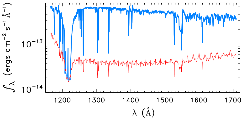
STAR0107-7251
