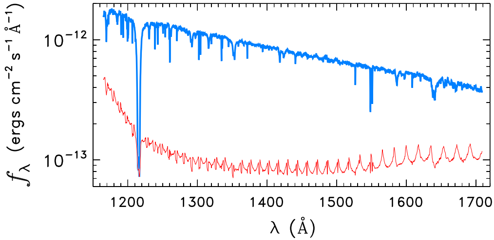
WD1159-034
