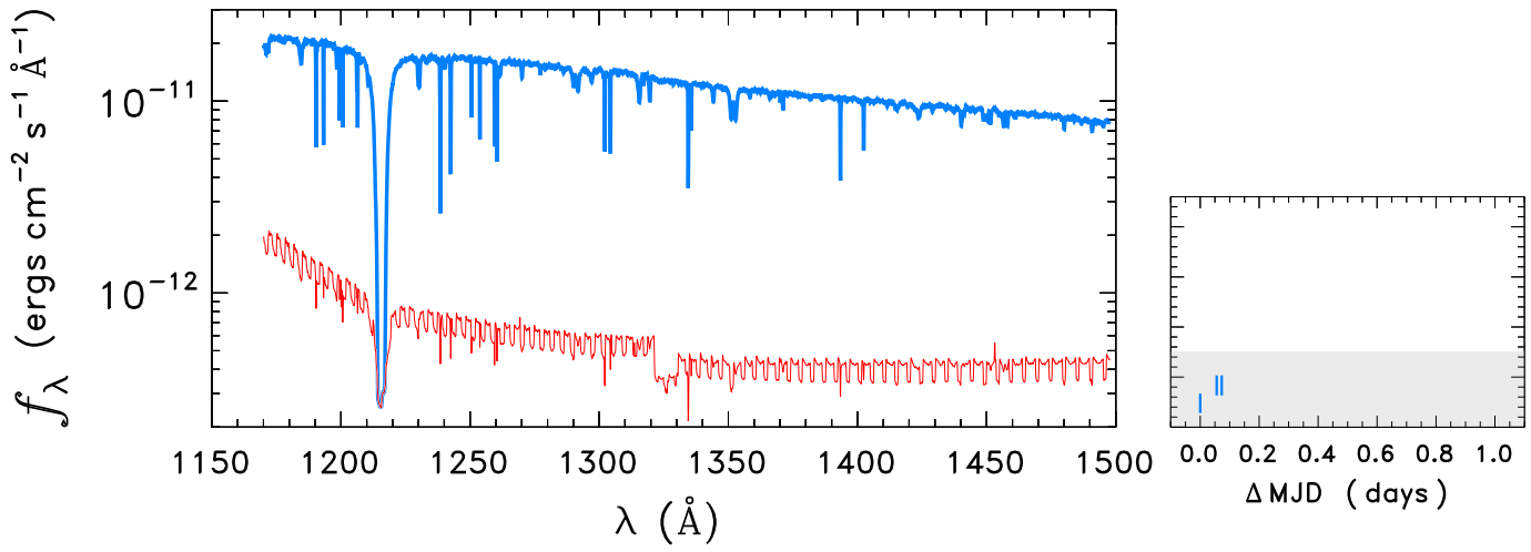
WD0044-121
