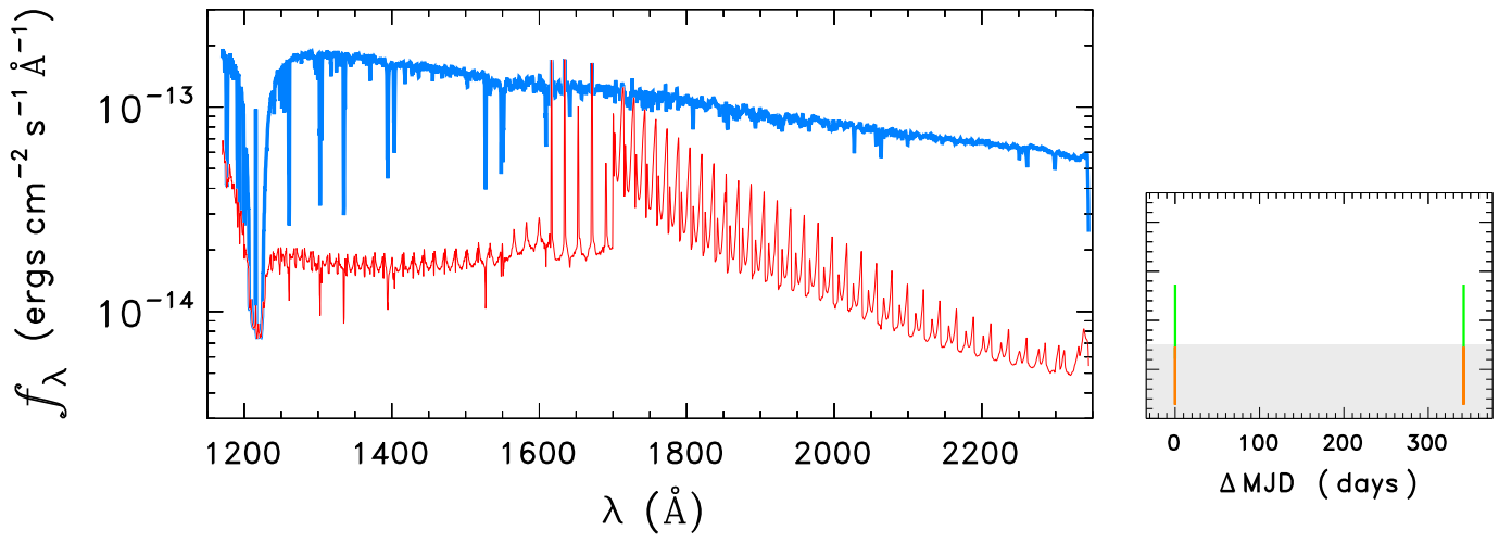
STAR0058-7244
