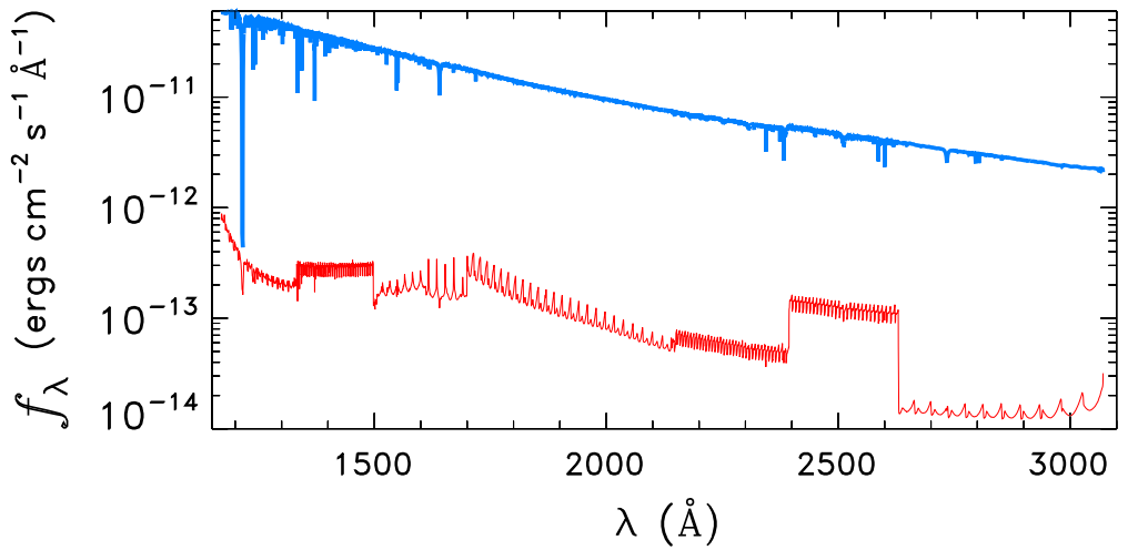
WD2148+286
