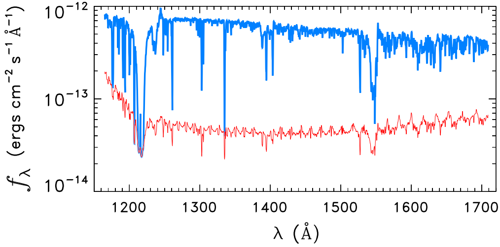
STAR0103-7202
