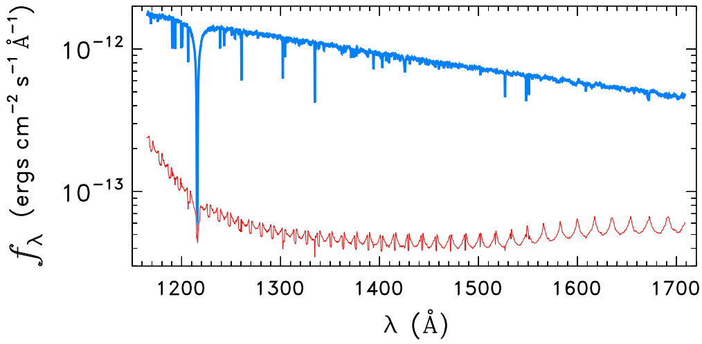
WD0556-375
