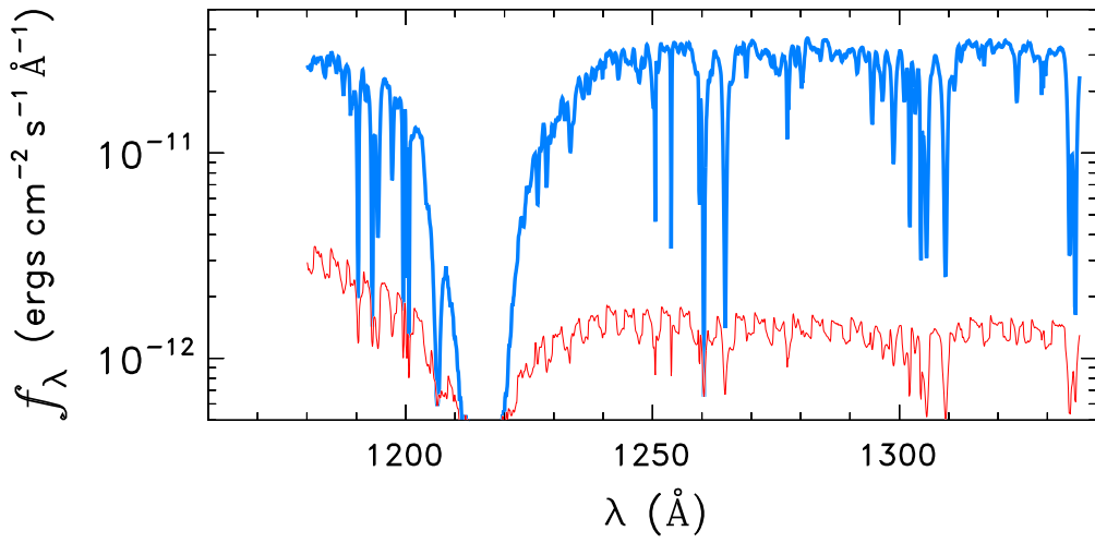
HD140037
