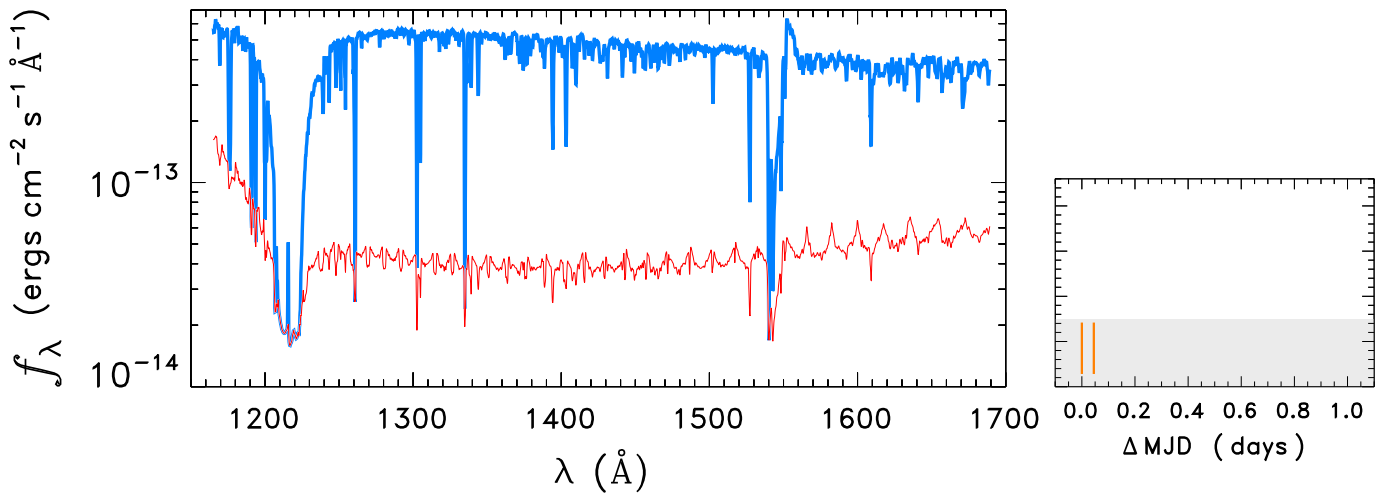
STAR0050-7253
