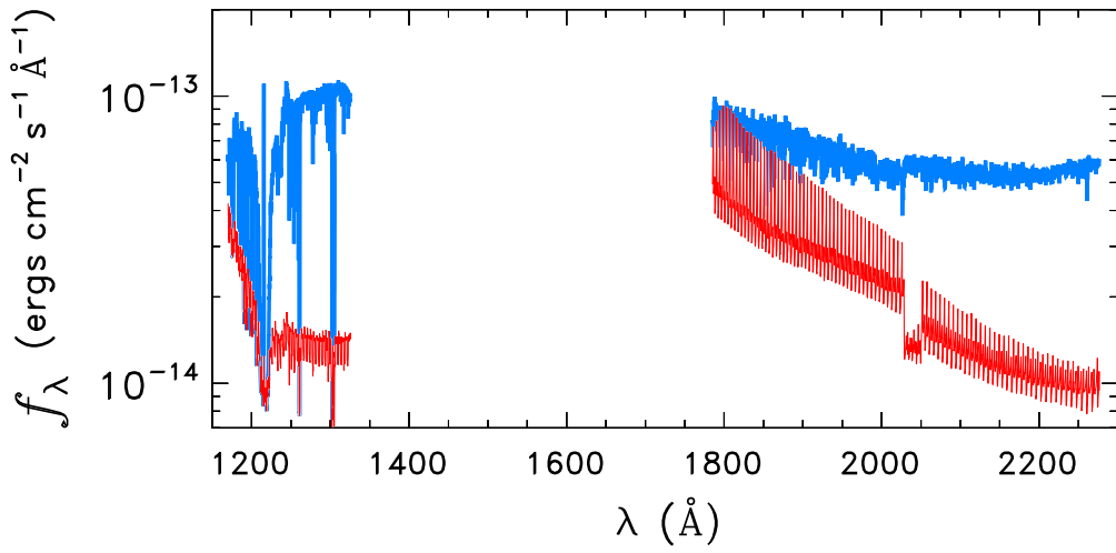
STAR0110-7242
