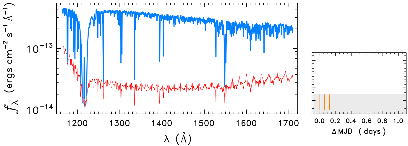
STAR0055-7317
