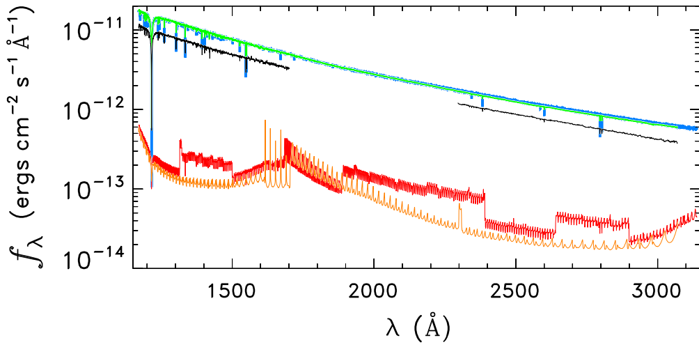
WD0501+527
