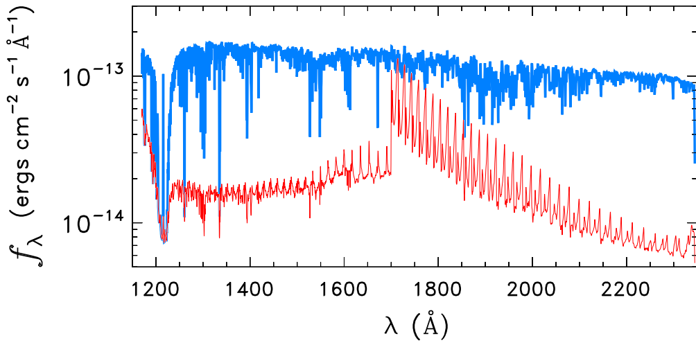
STAR0056-7228
