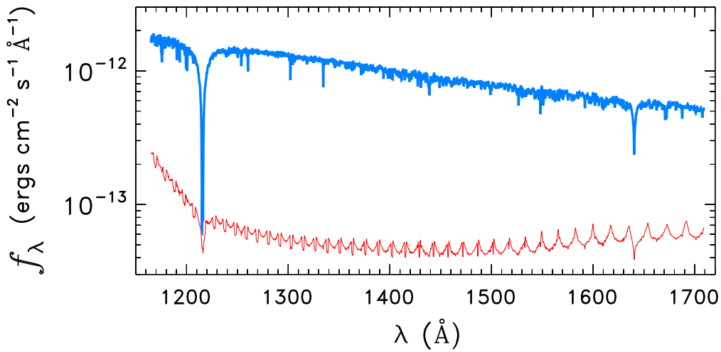
WD1210+533
