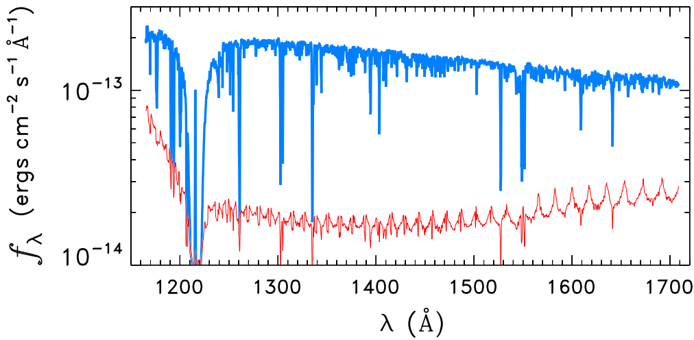
STAR0058-7210b
