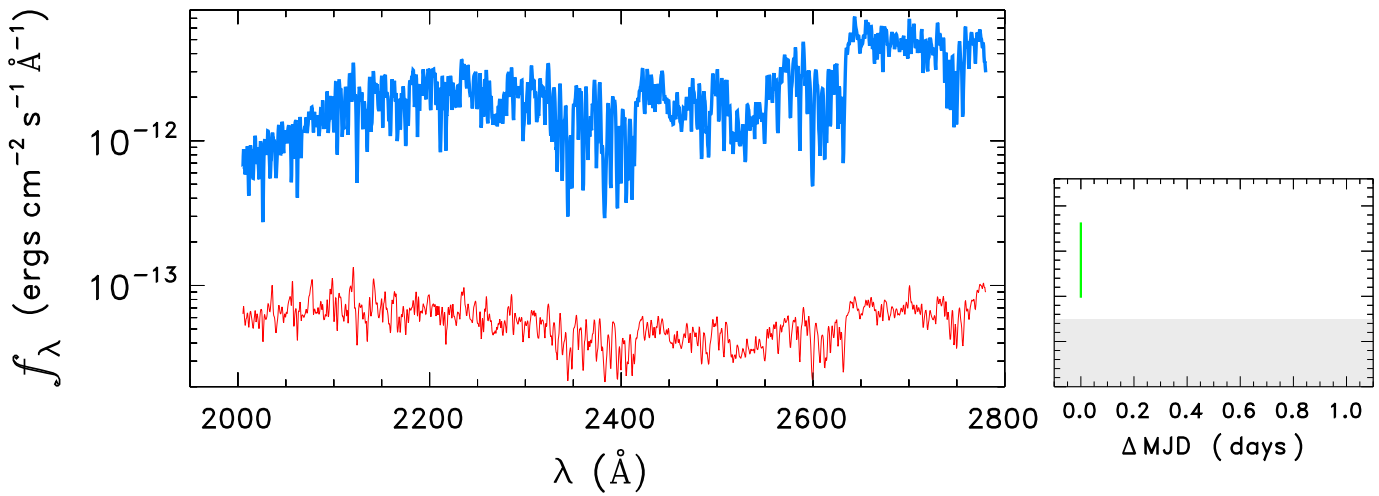
HD43318
