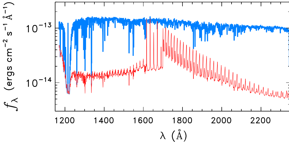
STAR0056-7227b
