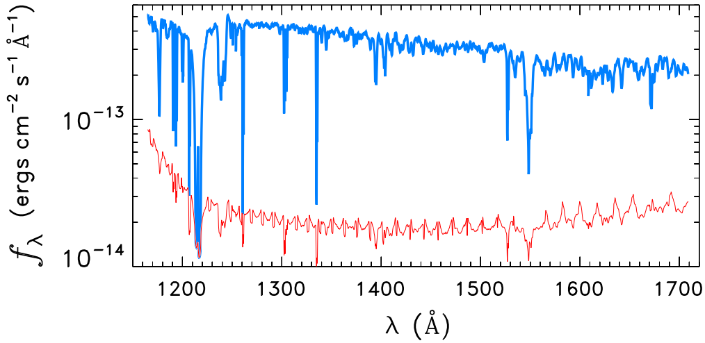
STAR0532-6622
