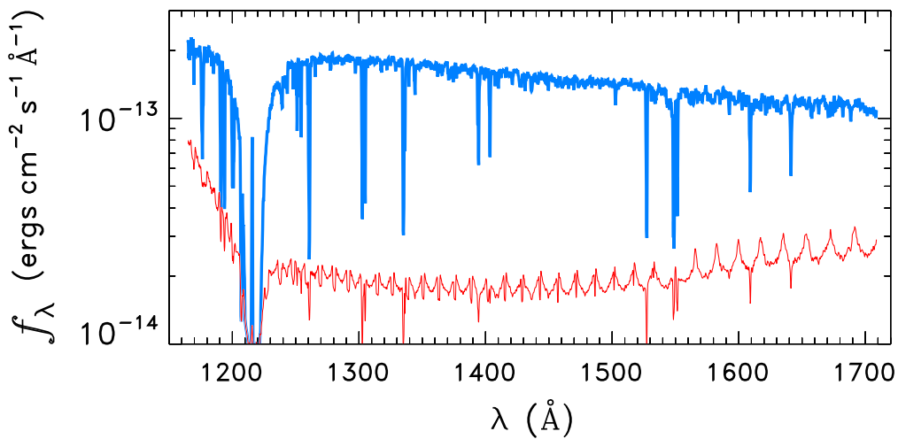
STAR0059-7210d
