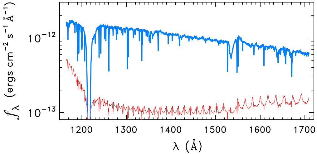
WD2134+125
