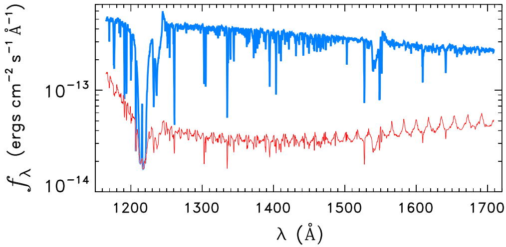
STAR0059-7210b
