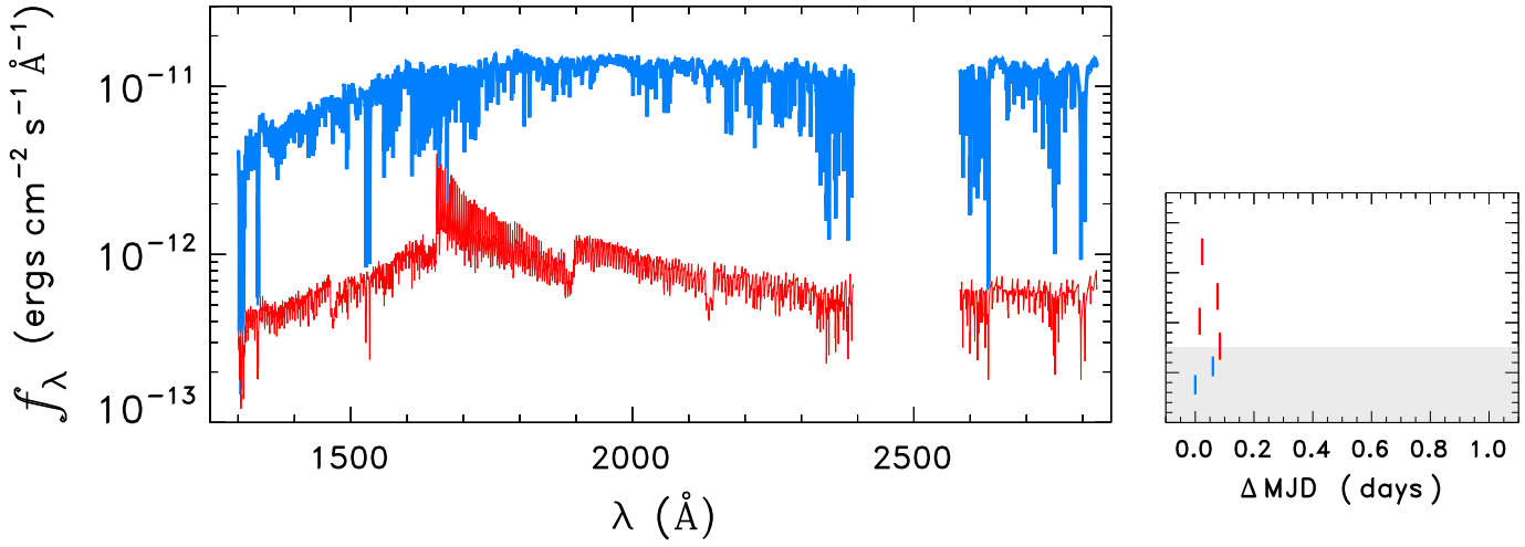
HD42111
