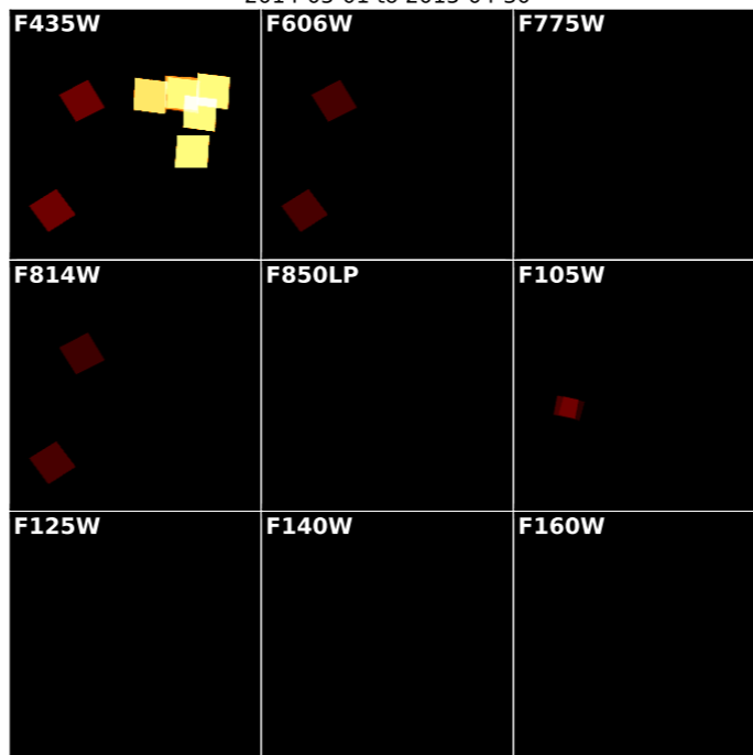
Misc. Programs
