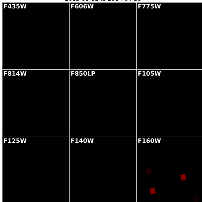
Misc. Programs
