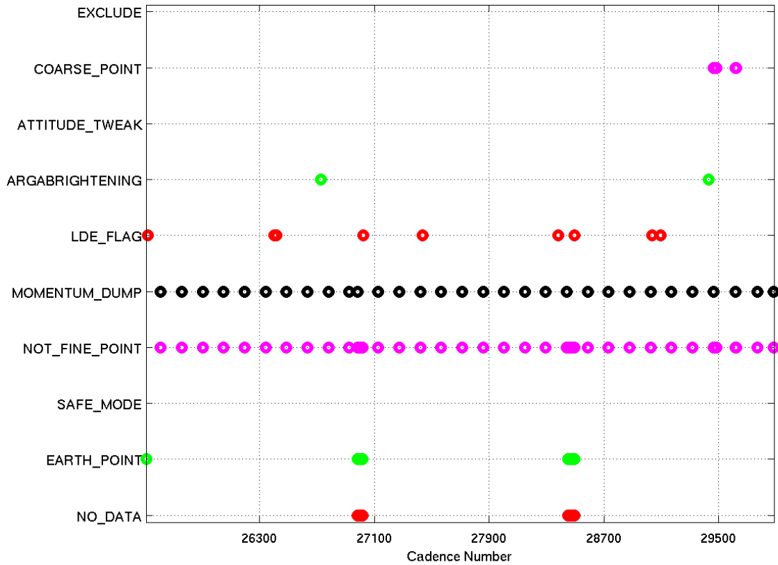
Figure 12: An overview of the location of the data anomalies flagged in Q7. ARGABRIGHTENING refers to cadences where the multiple-channel Argabrightening flag (flag 0x07, decimal value 64) was set.
