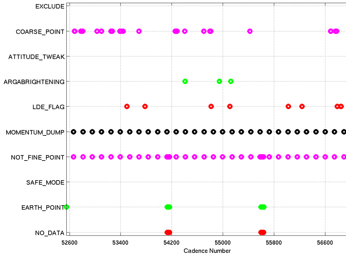
Figure 19: An overview of the location of the data anomalies flagged in Q13. ARGABRIGHTENING refers to cadences where the multiple-channel Argabrightening flag (flag 0x07, decimal value 64) was set.
