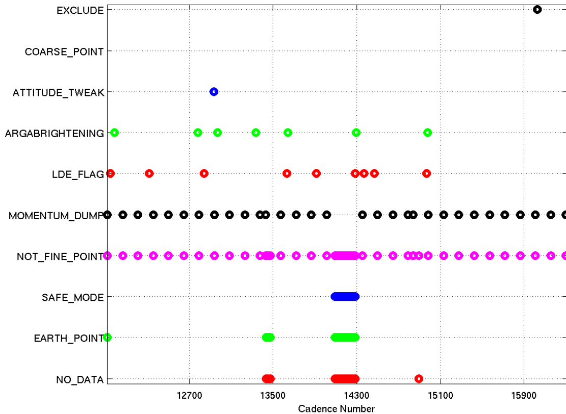
Figure 9: An overview of the location of the data anomalies flagged in Q4. ARGABRIGHTENING refers to cadences where the multiple-channel Argabrightening flag (flag 0x07, decimal value 64) was set.
