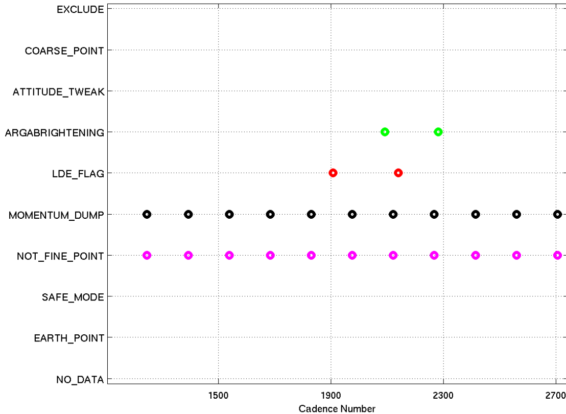
Figure 6: An overview of the location of the data anomalies flagged in Q1. ARGABRIGHTENING refers to cadences where the multiple-channel Argabrightening flag (flag 0x07, decimal value 64) was set.
