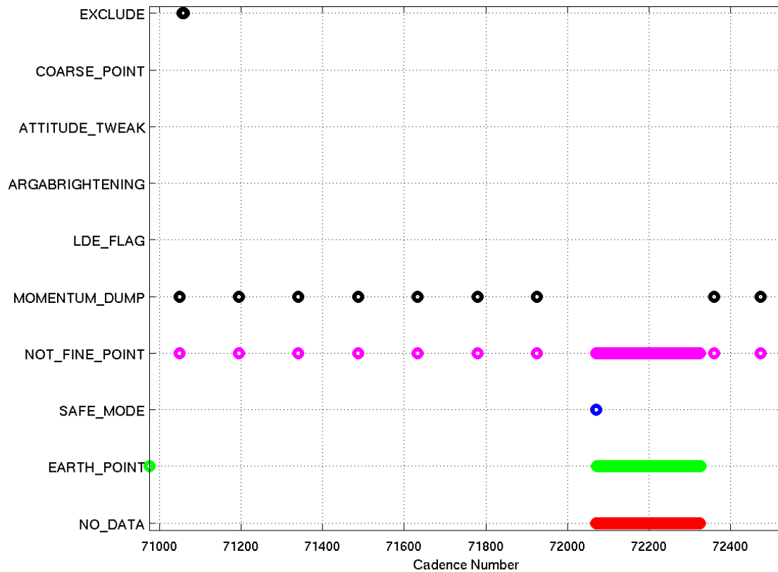
Figure 23: An overview of the location of the data anomalies flagged in Q17. ARGABRIGHTENING refers to cadences where the multiple-channel Argabrightening flag (flag 0x07, decimal value 64) was set.
