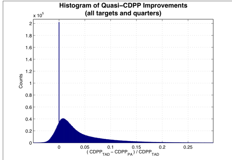
Figure 1: Histogram of fractional quasi-CDPP improvement when comparing light curves produced from revised PA apertures with those produced from the TAD apertures. Positive values indicate improved photometric precision. Note that each target is counted separately for each quarter. That is, the sum of the histogram values is the sum of all targets over all quarters.
