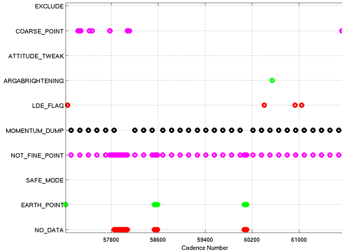
Figure 20: An overview of the location of the data anomalies flagged in Q14. ARGABRIGHTENING refers to cadences where the multiple-channel Argabrightening flag (flag 0x07, decimal value 64) was set.
