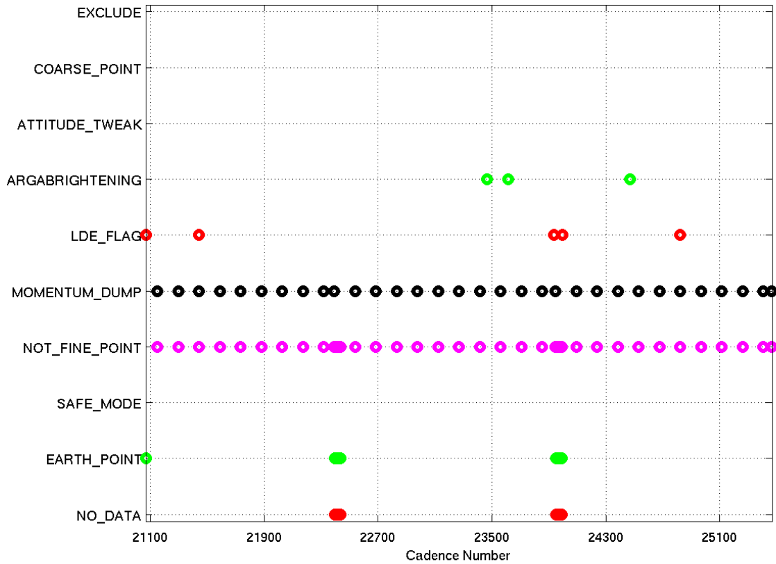
Figure 11: An overview of the location of the data anomalies flagged in Q6. ARGABRIGHTENING refers to cadences where the multiple-channel Argabrightening flag (flag 0x07, decimal value 64) was set.
