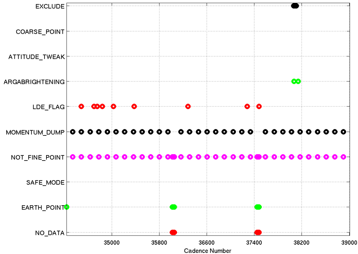
Figure 14: An overview of the location of the data anomalies flagged in Q9. ARGABRIGHTENING refers to cadences where the multiple-channel Argabrightening flag (flag 0x07, decimal value 64) was set.
