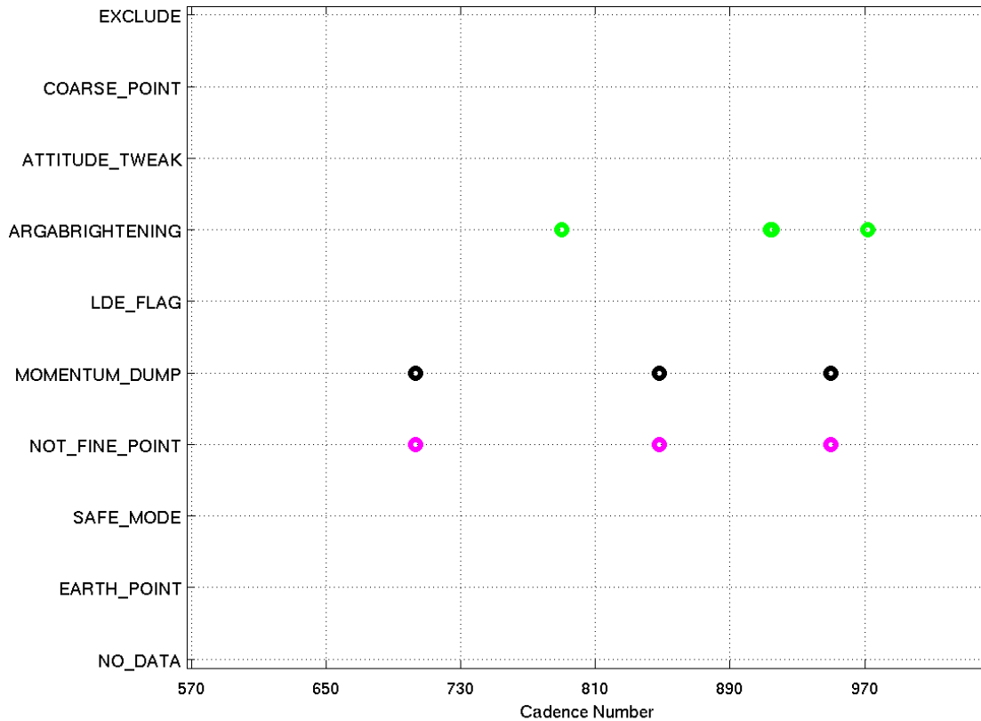
Figure 5: An overview of the location of the data anomalies flagged in Q0. ARGABRIGHTENING refers to cadences where the multiple-channel Argabrightening flag (flag 0x07, decimal value 64) was set.
