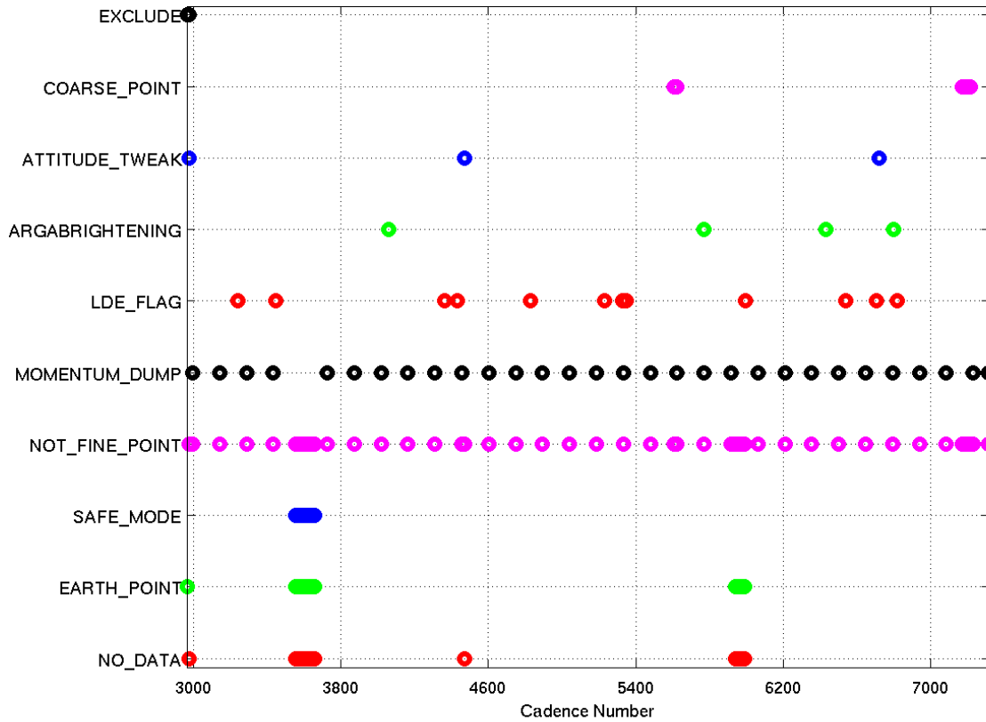
Figure 7: An overview of the location of the data anomalies flagged in Q2. ARGABRIGHTENING refers to cadences where the multiple-channel Argabrightening flag (flag 0x07, decimal value 64) was set.
