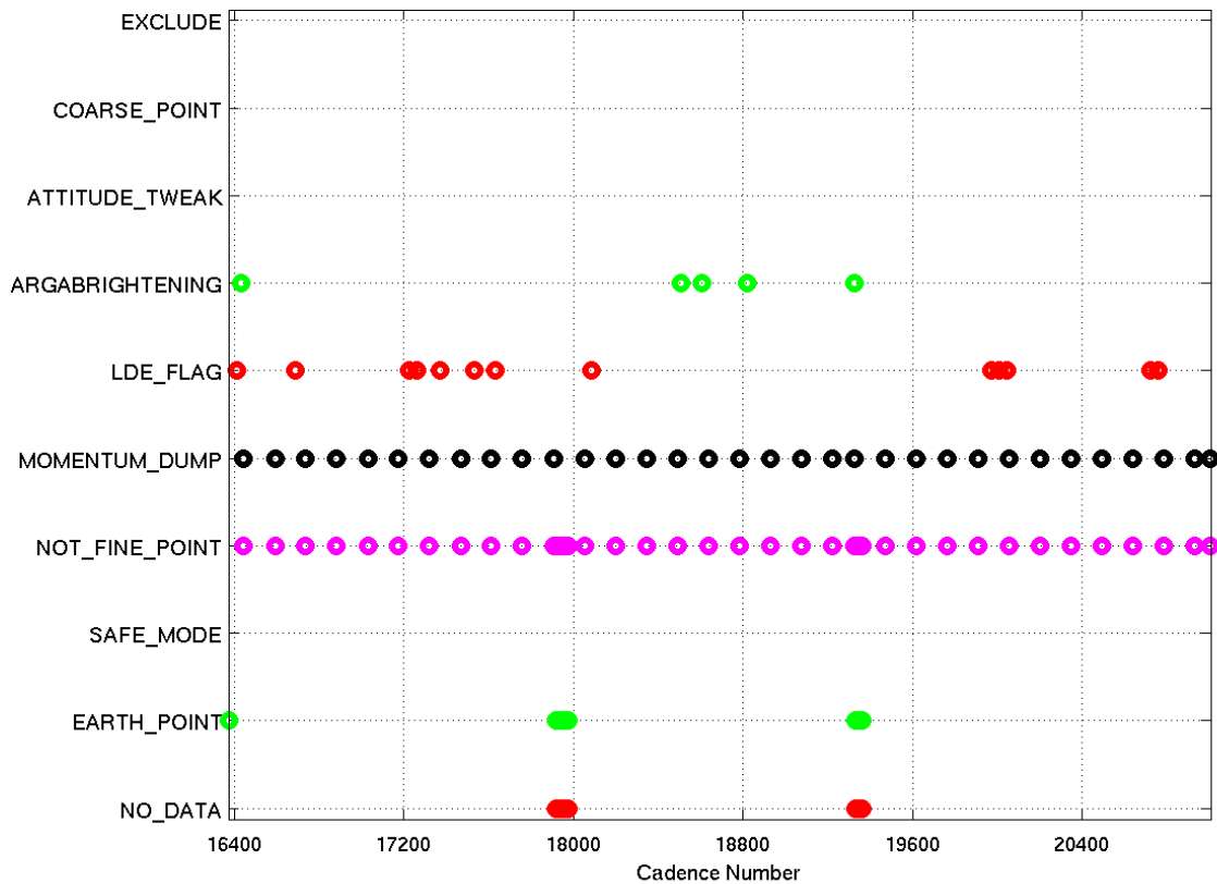
Figure 10: An overview of the location of the data anomalies flagged in Q5. ARGABRIGHTENING refers to cadences where the multiple-channel Argabrightening flag (flag 0x07, decimal value 64) was set.
