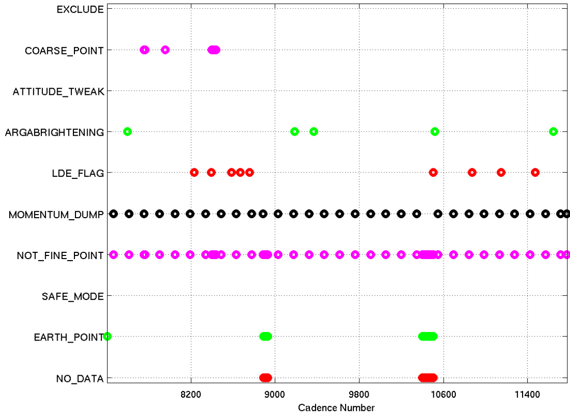
Figure 8: An overview of the location of the data anomalies flagged in Q3. ARGABRIGHTENING refers to cadences where the multiple-channel Argabrightening flag (flag 0x07, decimal value 64) was set.
