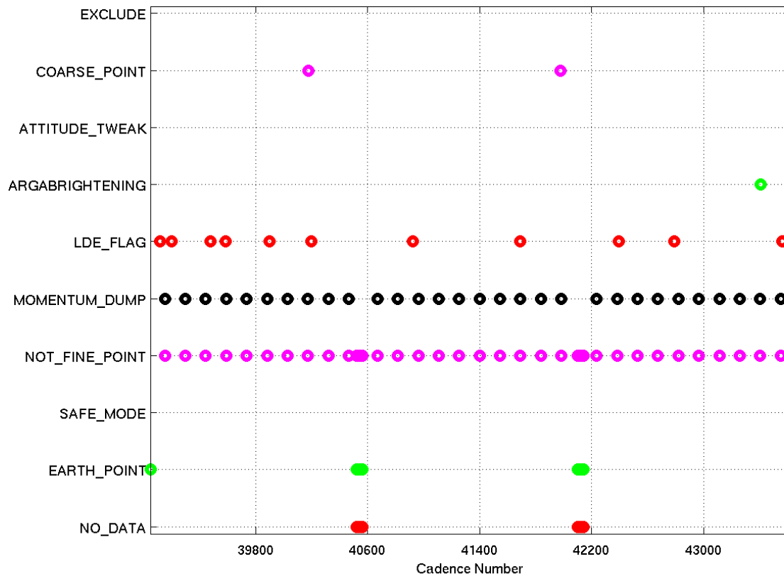
Figure 15: An overview of the location of the data anomalies flagged in Q10. ARGABRIGHTENING refers to cadences where the multiple-channel Argabrightening flag (flag 0x07, decimal value 64) was set.
