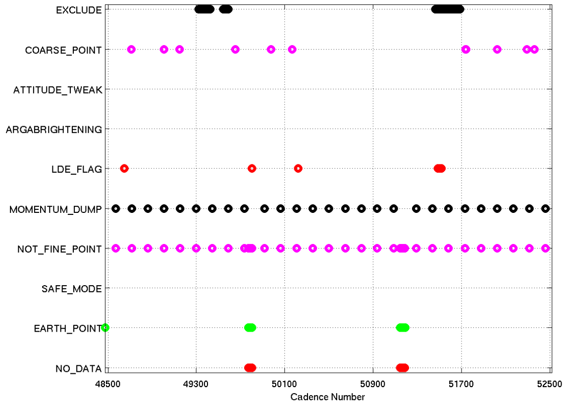
Figure 17: An overview of the location of the data anomalies flagged in Q12. ARGABRIGHTENING refers to cadences where the multiple-channel Argabrightening flag (flag 0x07, decimal value 64) was set.
