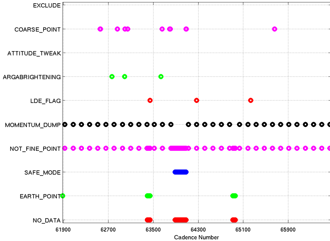
Figure 21: An overview of the location of the data anomalies flagged in Q15. ARGABRIGHTENING refers to cadences where the multiple-channel Argabrightening flag (flag 0x07, decimal value 64) was set.
