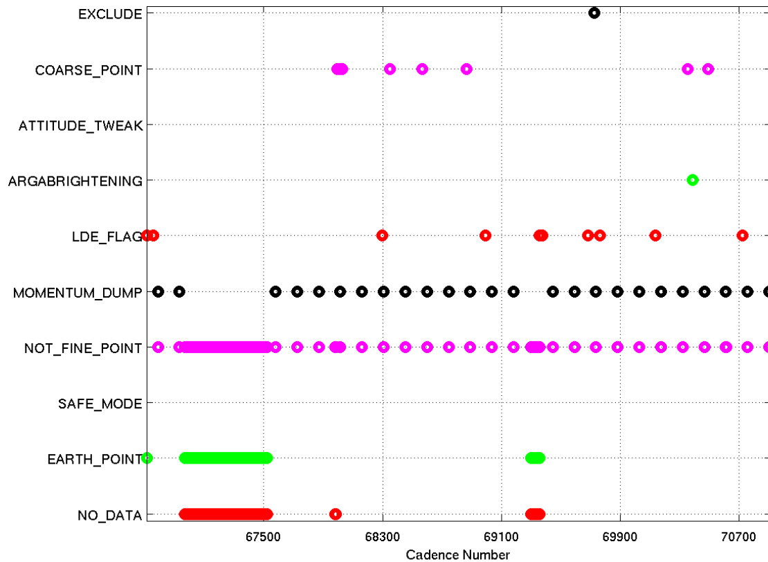
Figure 22: An overview of the location of the data anomalies flagged in Q16. ARGABRIGHTENING refers to cadences where the multiple-channel Argabrightening flag (flag 0x07, decimal value 64) was set.
