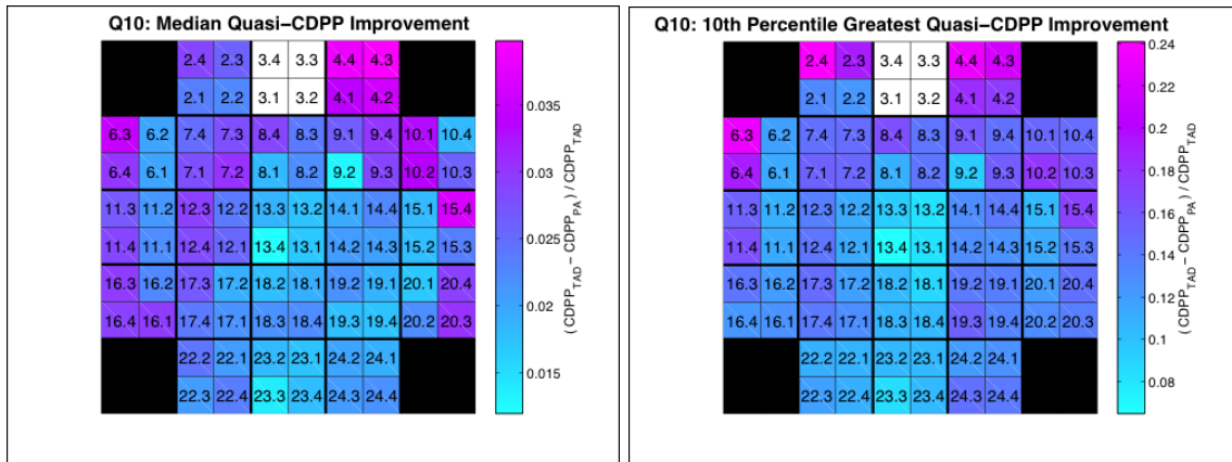
Figure 2: Spatial distribution of median (left) and top tenth percentile (right) quasi-CDPP improvement across the FOV in quarter 10. This spatial pattern is representative of the improvement seen in most quarters. In general, the largest improvements appear to be correlated with the most defocused stars.
