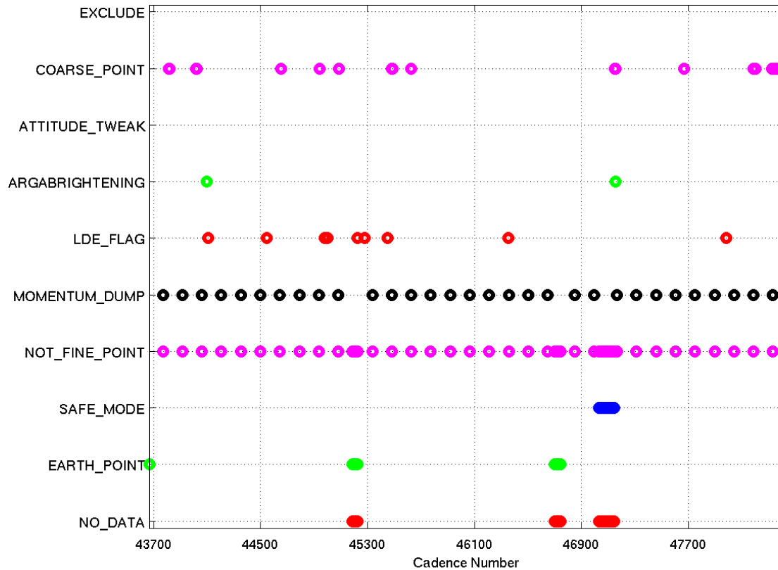
Figure 16: An overview of the location of the data anomalies flagged in Q11. ARGABRIGHTENING refers to cadences where the multiple-channel Argabrightening flag (flag 0x07, decimal value 64) was set.
