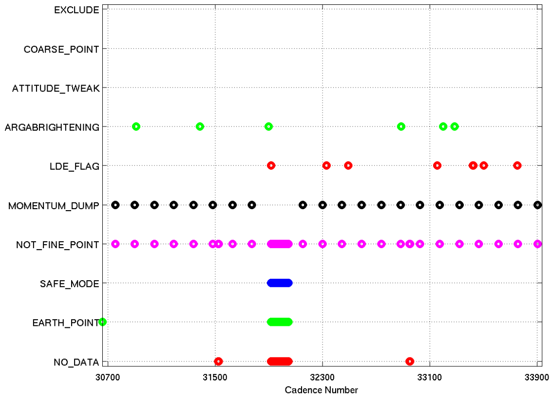
Figure 13: An overview of the location of the data anomalies flagged in Q8. ARGABRIGHTENING refers to cadences where the multiple-channel Argabrightening flag (flag 0x07, decimal value 64) was set.
