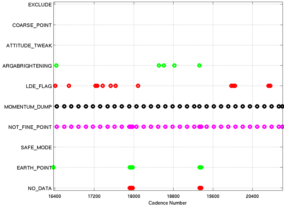
Figure 8: An overview of the location of the data anomalies flagged in Q5. ARGABRIGHTENING refers to cadences where the multiple-channel Argabrightening flag (flag 0x07, decimal value 64) was set.
